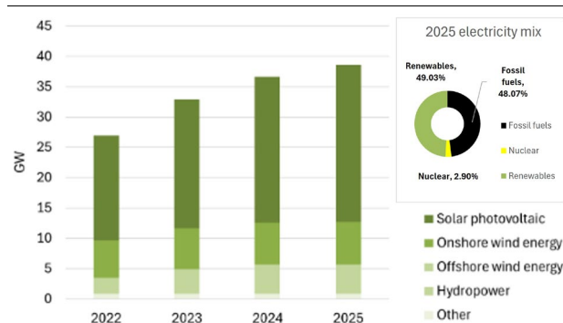
Graph A9.3: Netherlands's installed renewable capacity vs electricity generation mix
